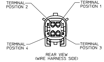
REAR VIEW (WIRE HARNESS SIDE)
